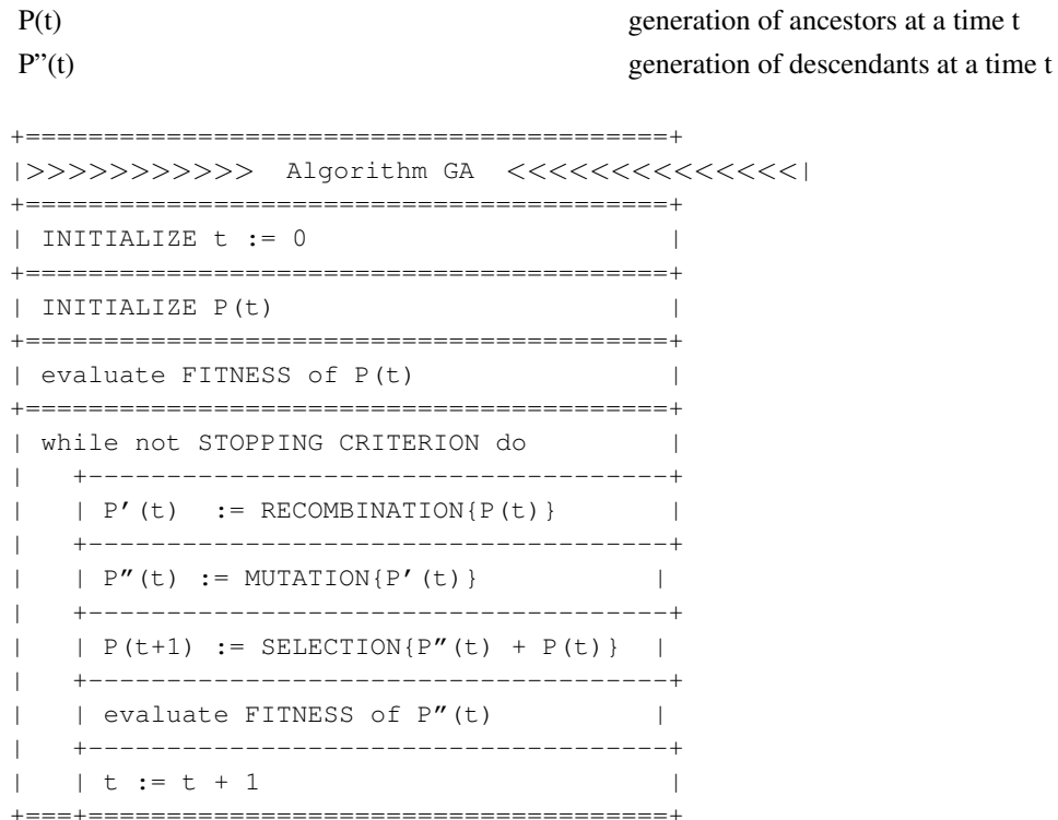
Figure 51-1. Structured Diagram of a Genetic Algorithm
