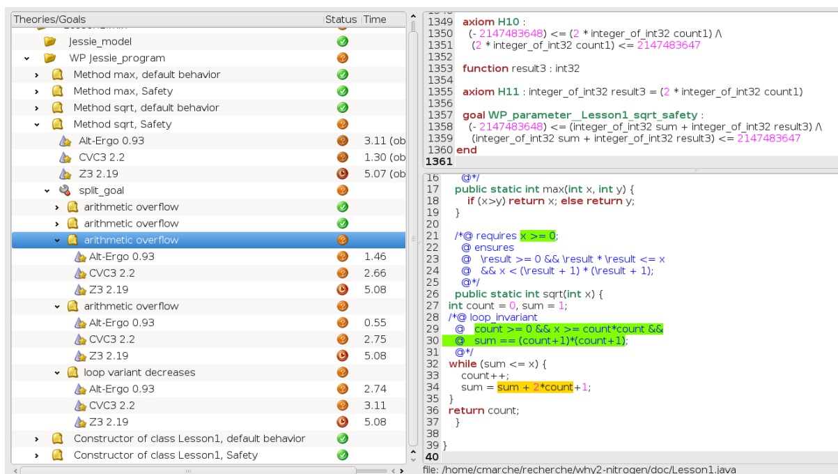
Figure 2.5: Safety VCs for sqrt
